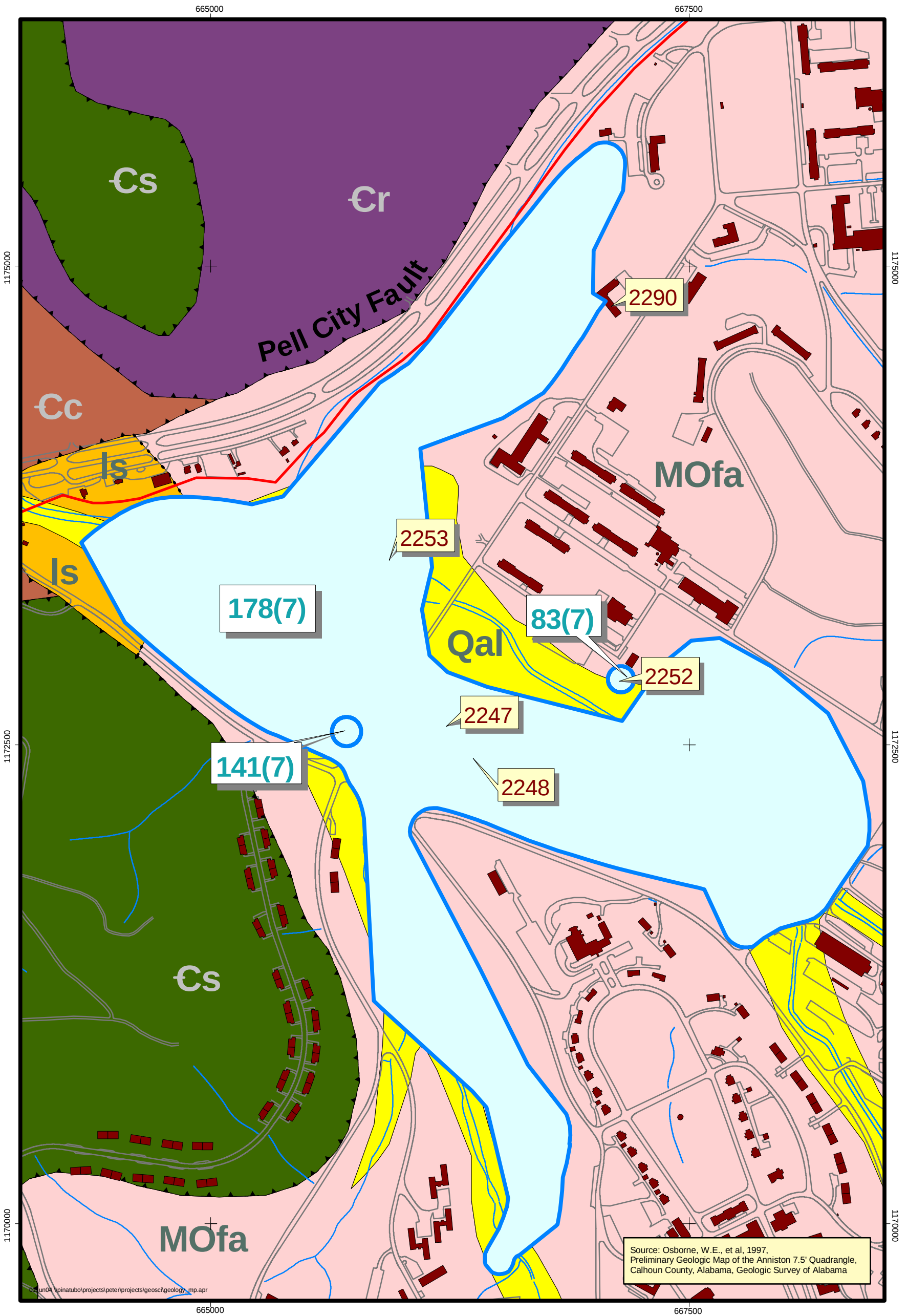
Figure 4-1 Geologic Map of the Golf Course, Parcels 178(7), 83(7), and 141(7)
